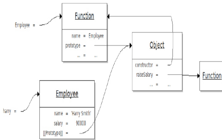
Figure 11-3 The constructor property
