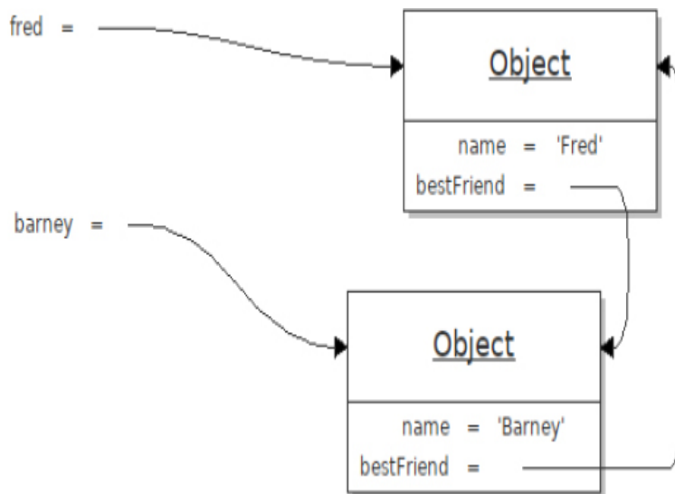
Figure 11-2 Circular references
